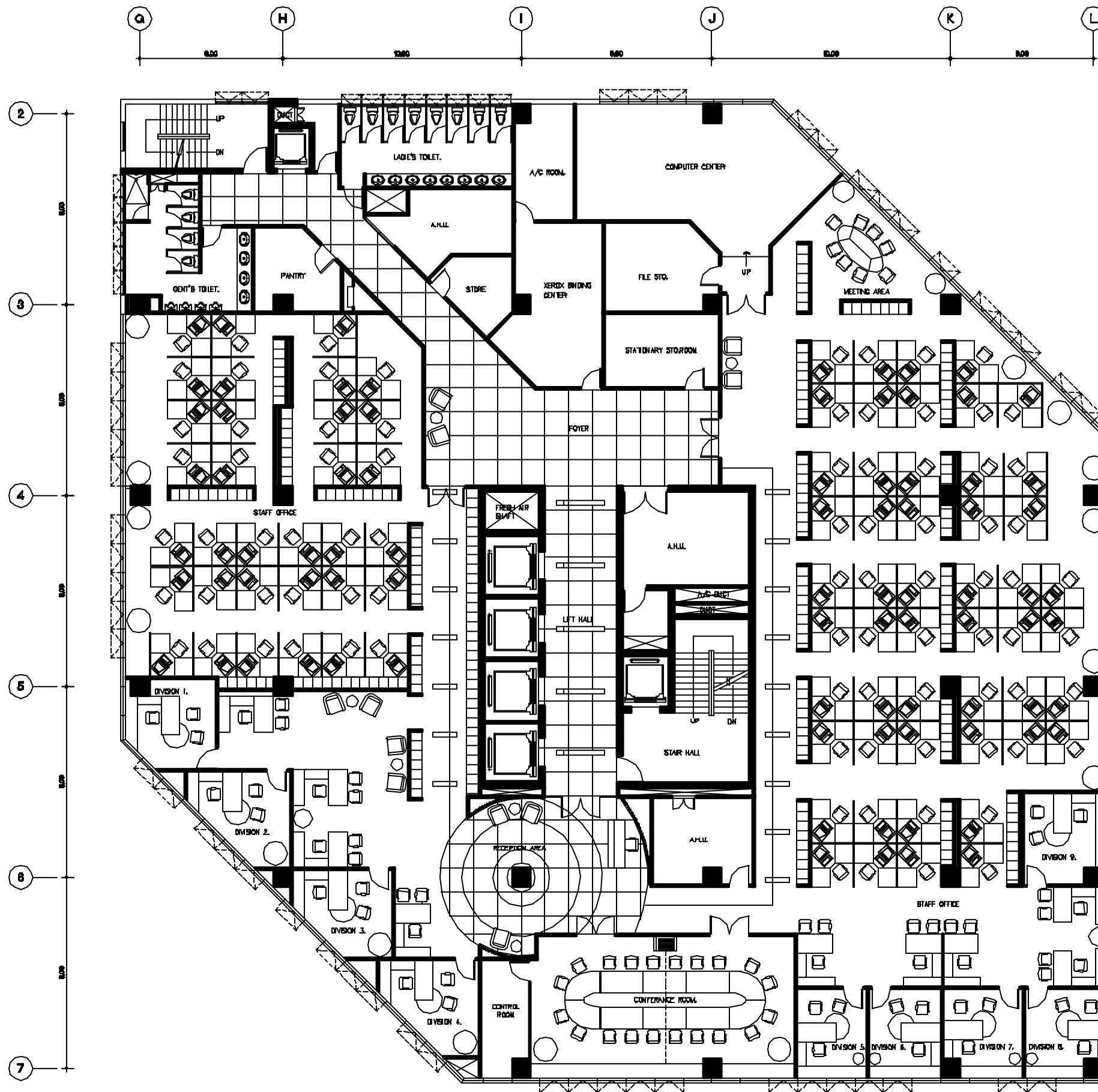
FURNITURE LAYOUT 15th PLAN
